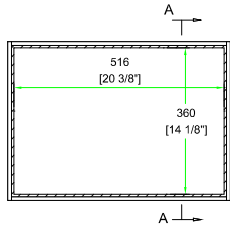
TOP VIEW OF COVER
