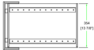
D-D VIEW
