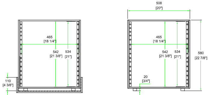
C-C VIEW
