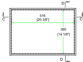
TOP VIEW OF BASE
