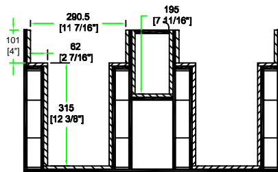
C-C VIEW
