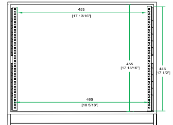
INSIDE VIEW
