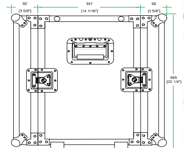
LEFT VIEW
