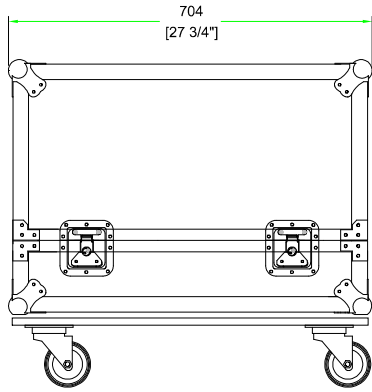
FRONT VIEW BACK VIEW
