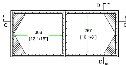
TOP VIEW OF BASE
