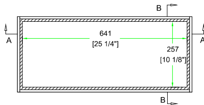
TOP VIEW OF COVER
