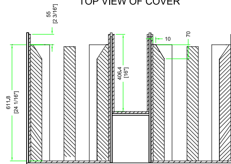
C-C VIEW
