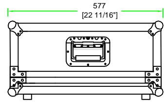
LEFT VIEW
