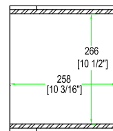
D-D VIEW
