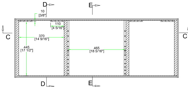
TOP VIEW OF BASE
