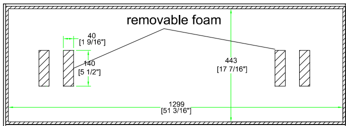
TOP VIEW OF COVER
