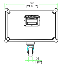
LEFT VIEW
