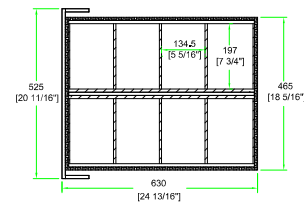
INSIDE VIEW OF 6WD
