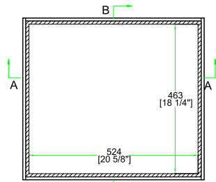
TOP VIEW OF COVER
