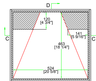
TOP VIEW OF BASE
