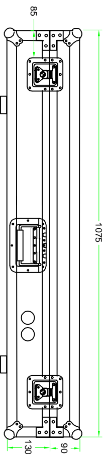
BACK VIEW
