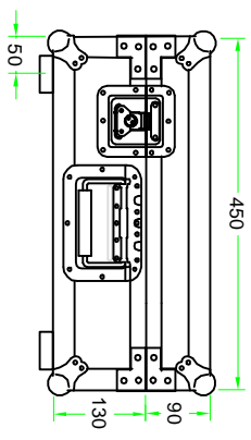
RIGHT VIEW
